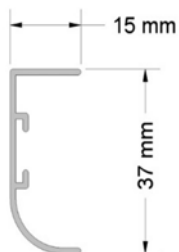
Guiding Channels
